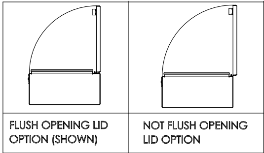
FLUSH OPENING LID OPTION (SHOWN) NOT FLUSH OPENING LID OPTION
