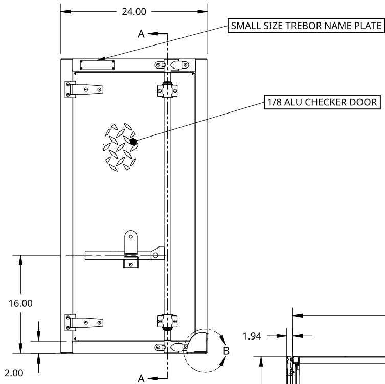
DRIVERS SIDE SCALE 1:16
