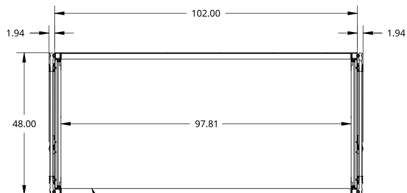
SECTION A - A SCALE 1:32
