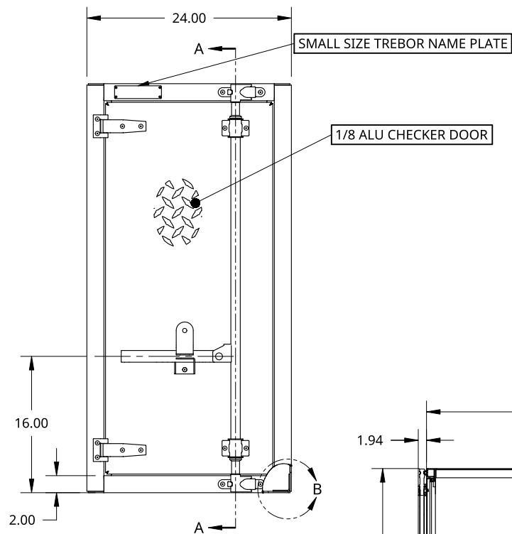
DRIVERS SIDE SCALE 1:16
